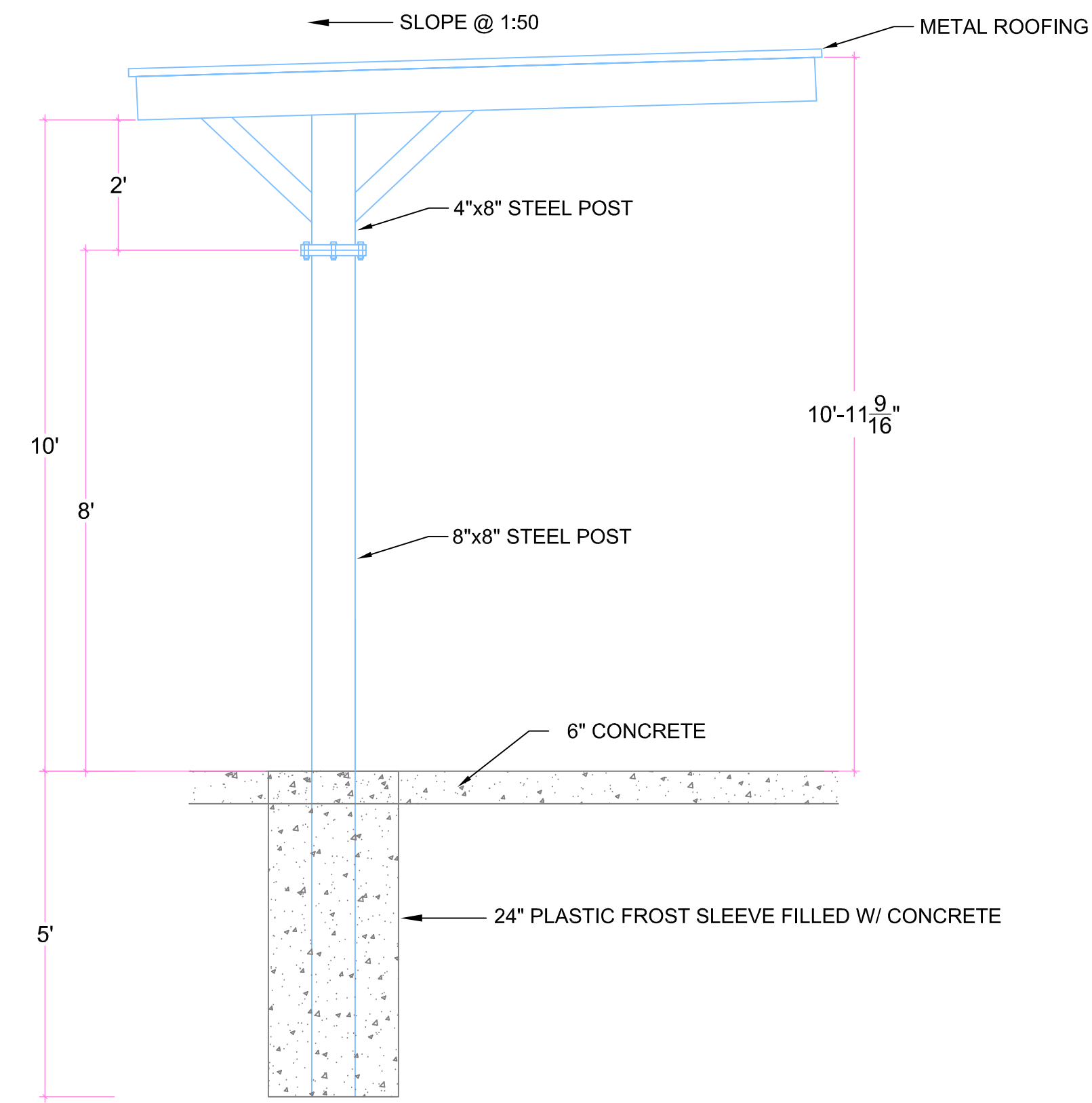
2 RIGHT VIEW - CANOPY STRUCTURE 1/8\"/>
