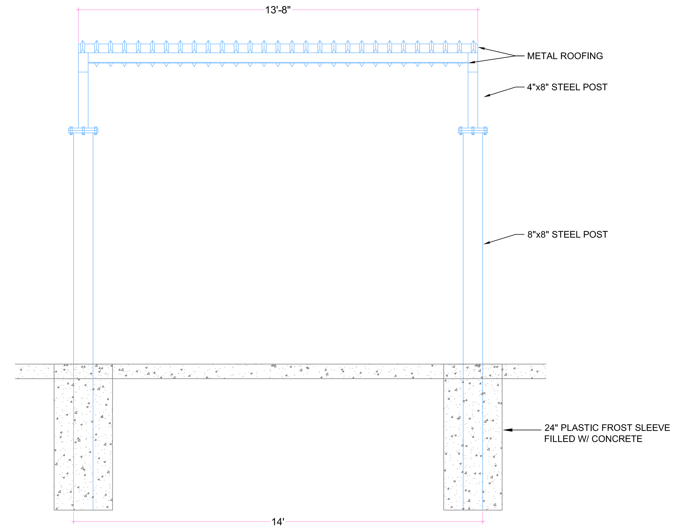
3 REAR VIEW - CANOPY STRUCTURE 1/8\"/>
