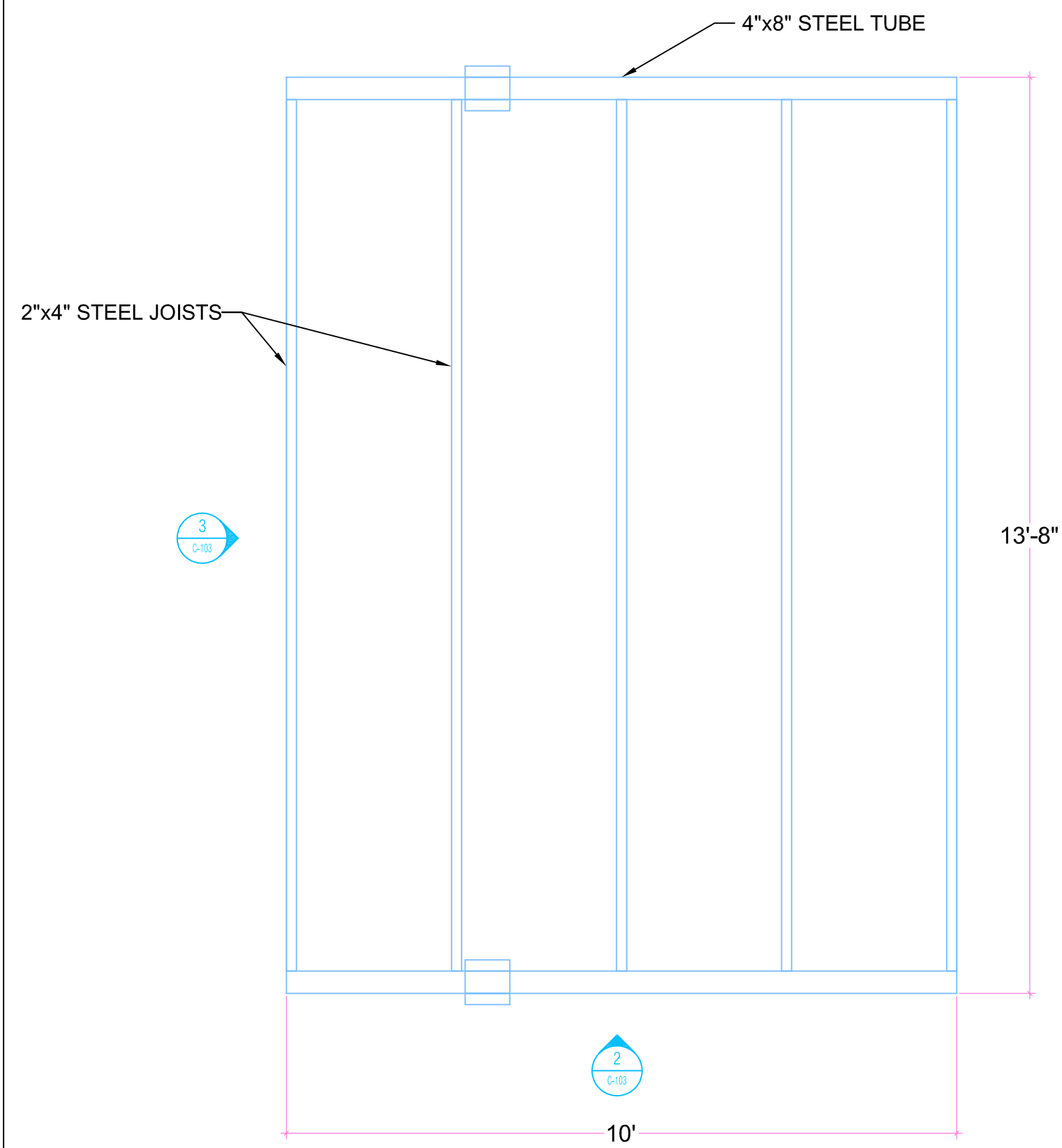
1 PLAN VIEW - CANOPY ROOF STRUCTURE 1/8\"/>
